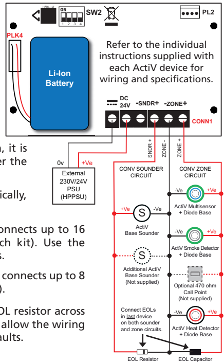
Fig.2 - Typical HAK/1 Hush-ActiV Connections
