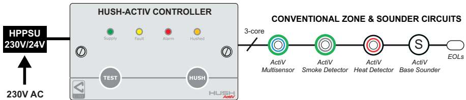
Fig.1 - Typical HAK/1 Hush-ActiV System
